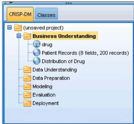
Figure 8. Vue CRISP-DM
