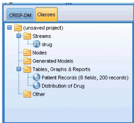
Figure 9. Vue Classes
